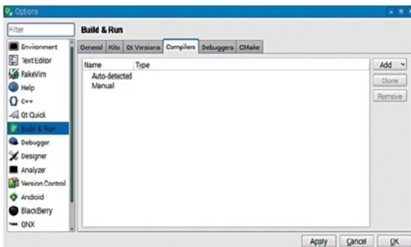
Fig. 1: Compilers window
