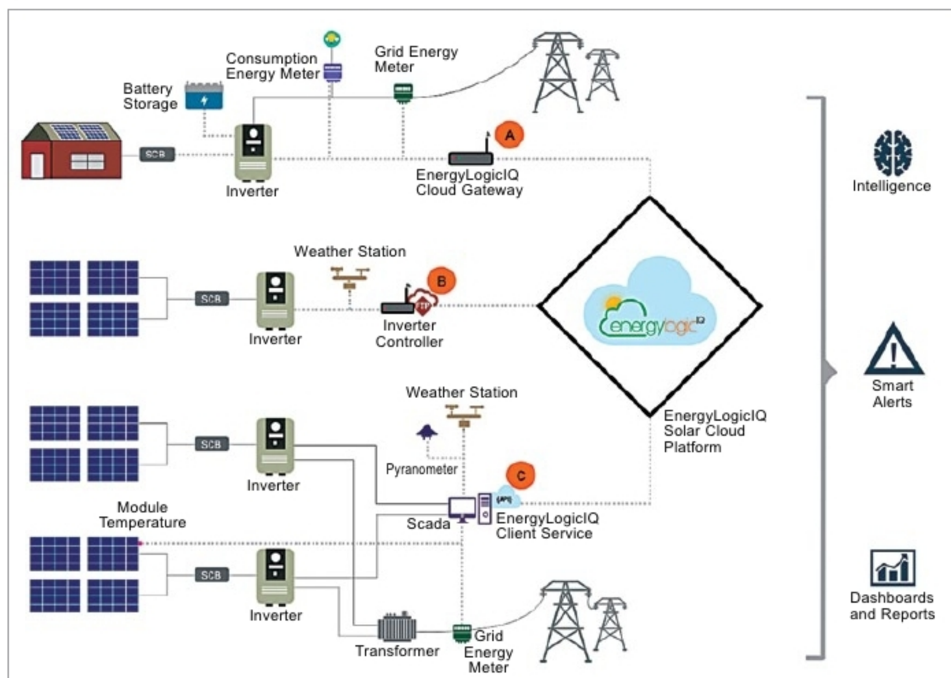
Solar energy monitoring system (Credit: www.logicladder.com )
