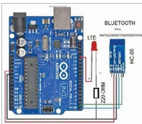
Fig. 20: Circuit diagram of Arduino with Bluetooth module
