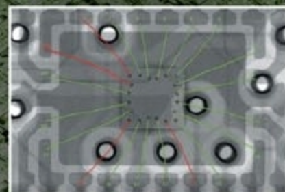
Wire-bond analysis
