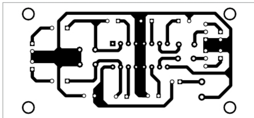
Fig. 3: Actual-size PCB layout of 5W stereo audio amplifier
