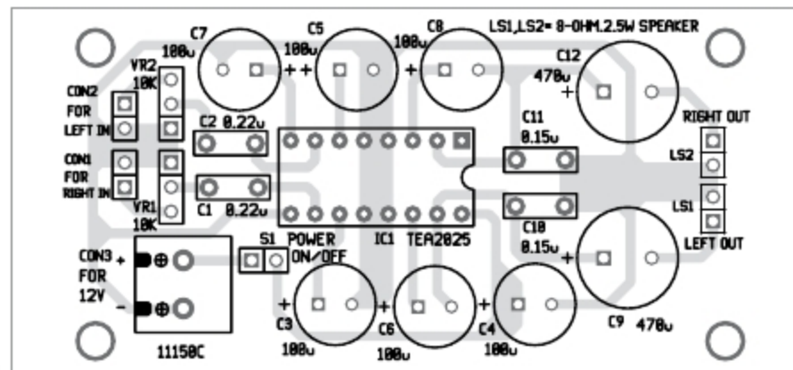
Fig. 4: Components layout for the PCB
