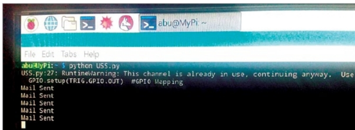
Fig. 3: Terminal window
