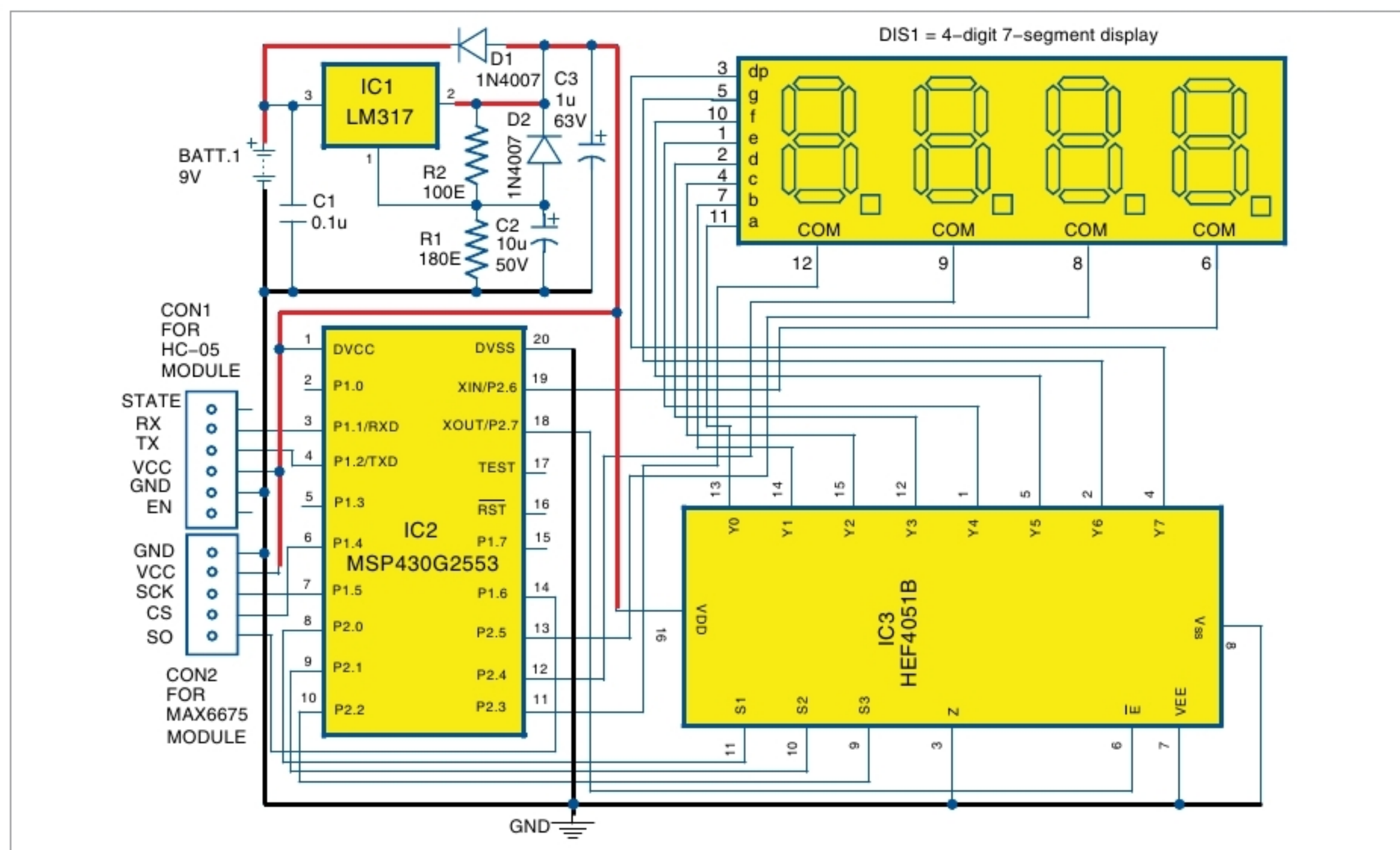
Fig. 3: Circuit diagram of the temperature measurement system
