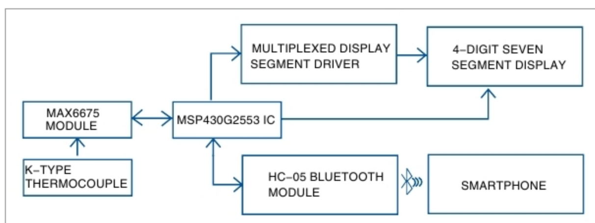
Fig. 2: Block diagram of the temperature measurement system
