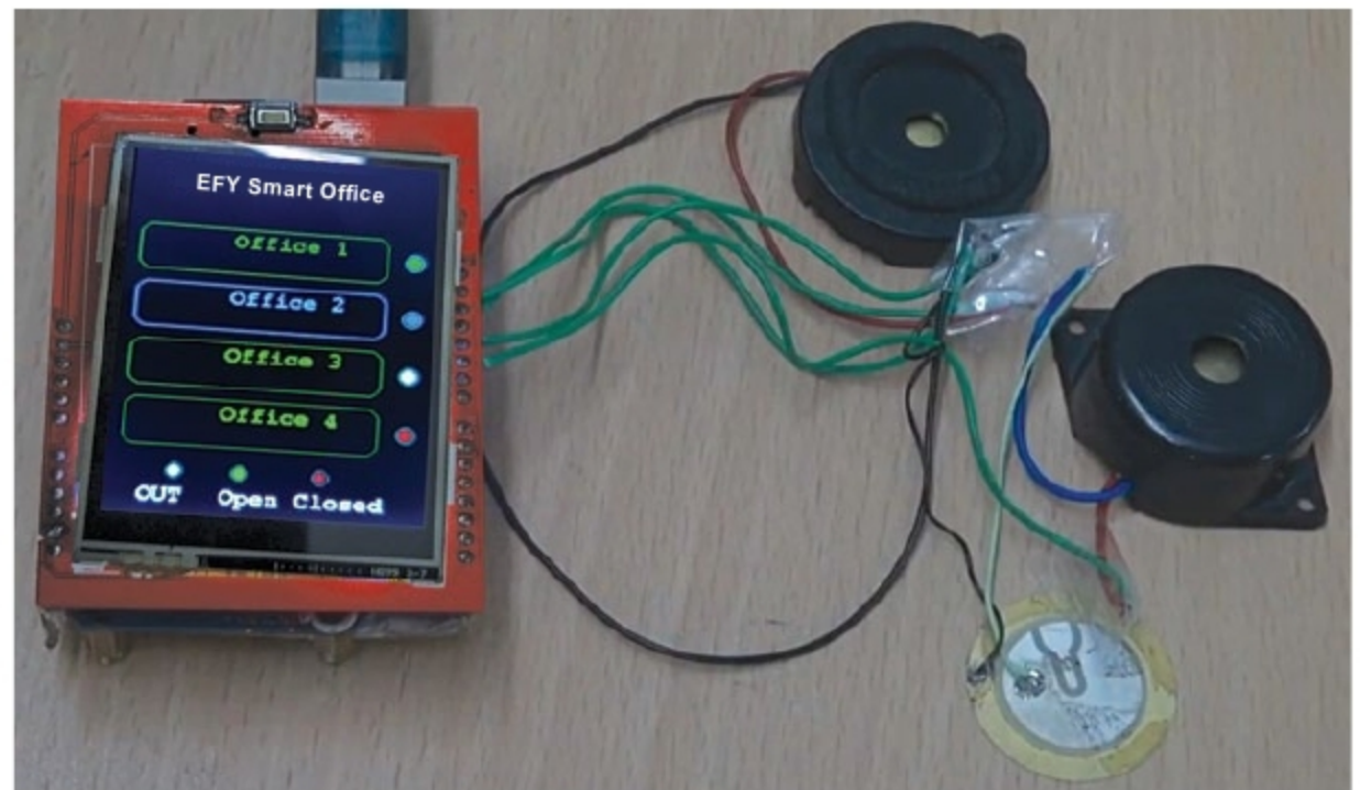
Fig. 1: Author's prototype
