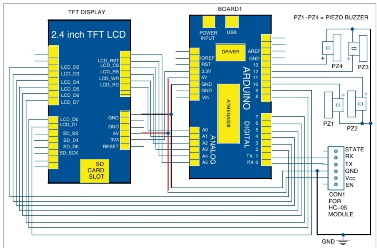
Fig. 2: Circuit diagram of the smart touch-controlled multi-doorbell system
