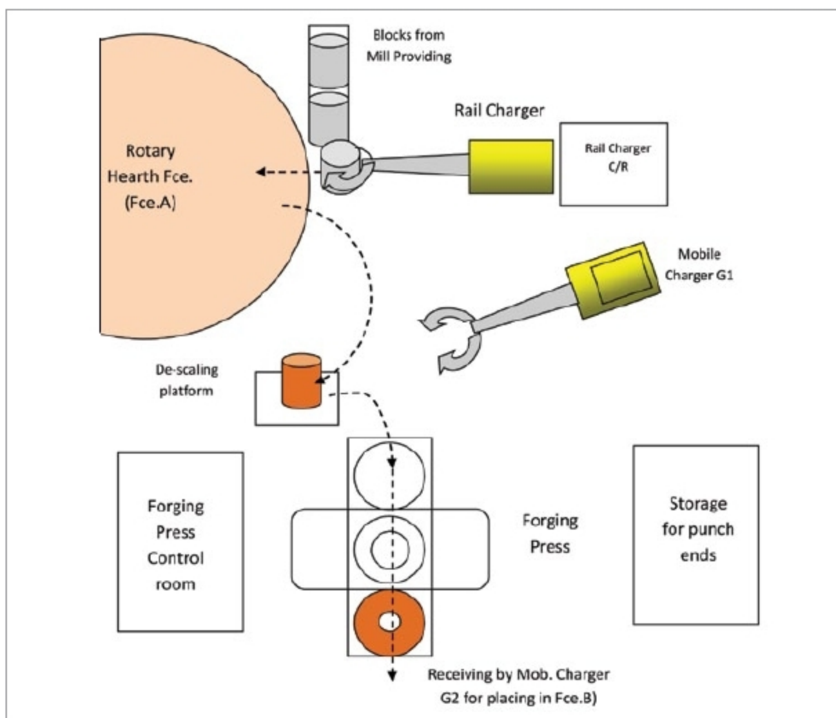
Fig. 4: Schematic layout for the wheel forging process
