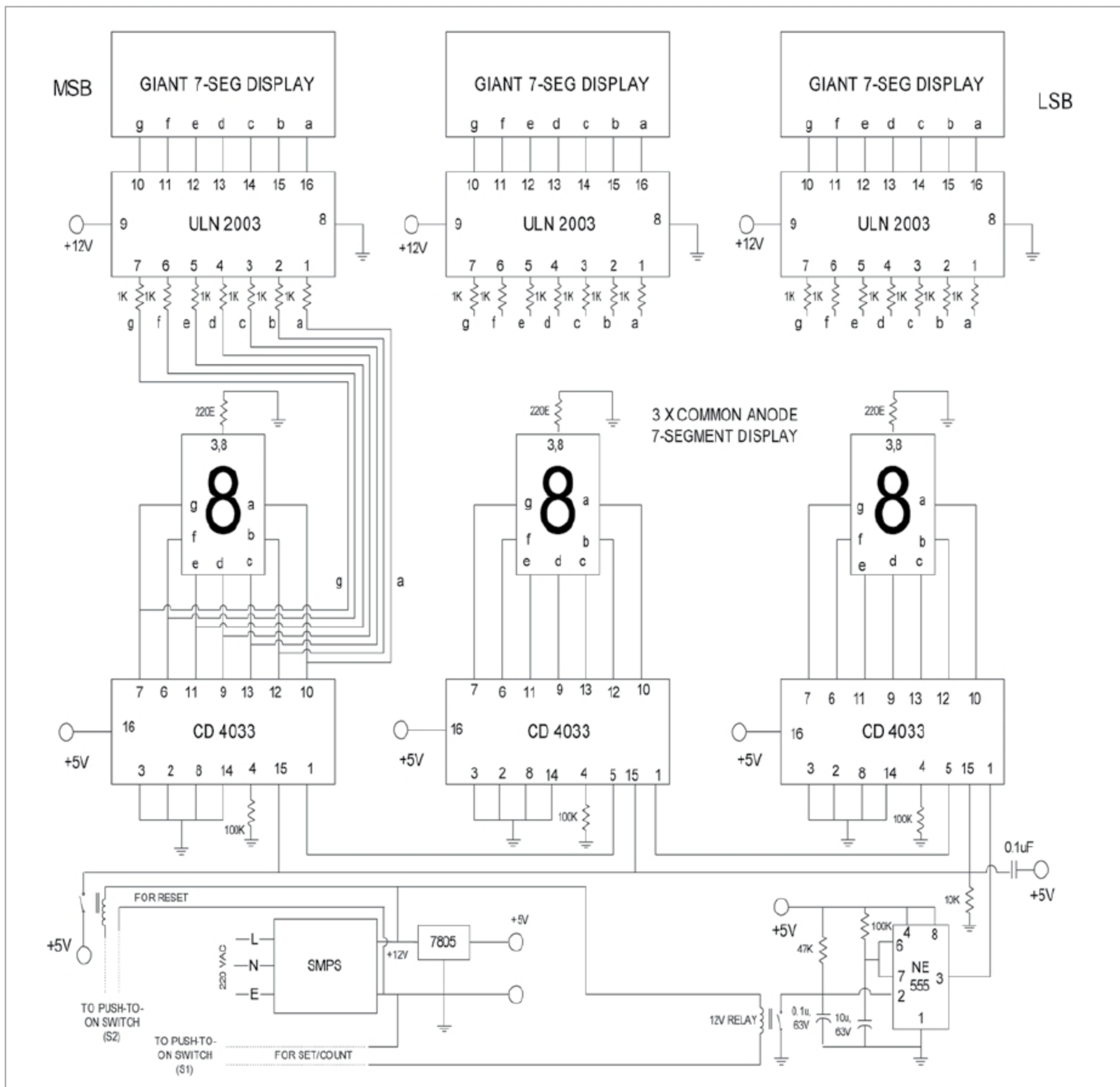
Fig. 6: Circuit diagram of three-digit digital wheel counter
