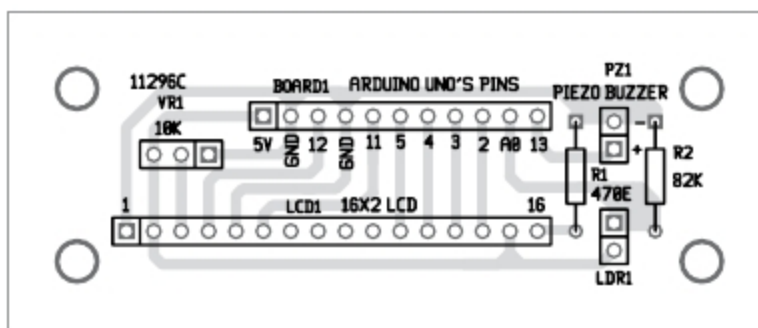
Fig. 3: Components layout for the PCB
