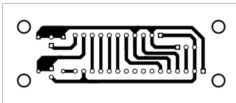
Fig. 2: Actual-size PCB layout of the light-level monitoring system
