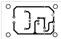
Fig. 3: Actual-size PCB layout of optical slave flash trigger
