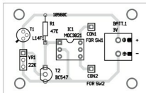
Fig. 4: Components layout for the PCB
