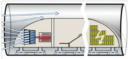
A pod would move through the tube with an air compressor on the front, passenger compartment in the middle and battery compartment at the back (Source: www.jebiga.com )
