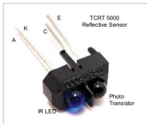
Fig. 5: Pin configuration of TCRT5000 sensor
