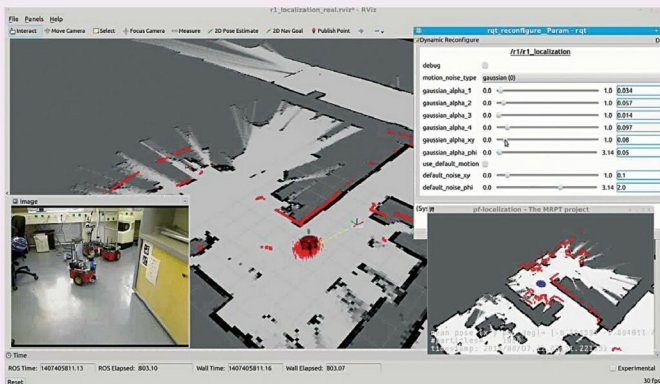
Fig. 1: MRPT particle filter localisation using ROS
