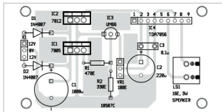
Fig. 4: Components layout for the PCB
