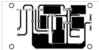
Fig. 3: Actual-size PCB layout of the 3W audio amplifier
