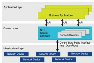
Fig. 5: SDN architecture components
