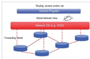
Fig. 7: Controlling mechanism in SDN (Courtesy: www.ieit.cnr.it)
