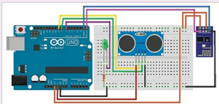
Fig. 1: Illustration of Fritzing through Breadboard view (Image courtesy: http://fritzing.org )
