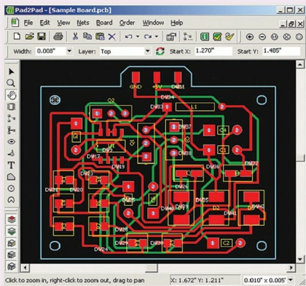
Fig. 2: Pad2Pad screen and layout (Image courtesy: www.brothersoft.com)
