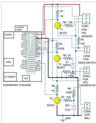
Fig. 2: Circuit of the IoT based notification system using RPi
