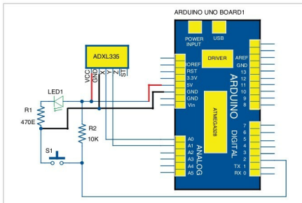
Fig. 2: Circuit diagram of the duck hunt game using Arduino Uno
