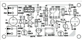
Fig. 4: Components layout of the PCB
