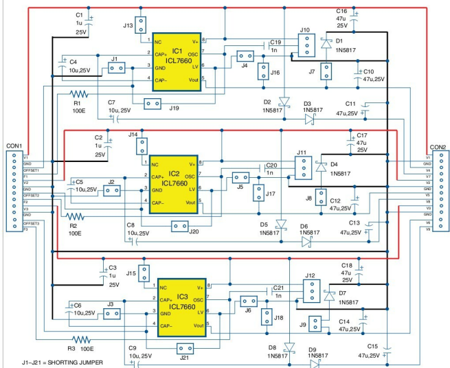
Fig. 1: Circuit diagram of the configurable DC-DC converter module
