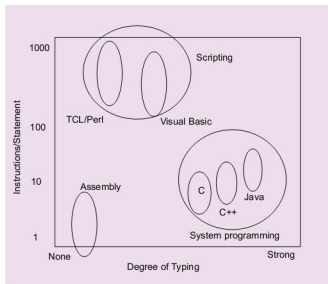
Fig. 3: Functionalities of different computer languages
