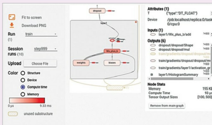
Fig. 3: Graphs and statistics on TensorFlow
