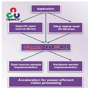
Fig. 8: OpenCV and OpenVX to accelerate vision system development
