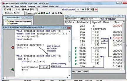
Fig. 3: Use of pointer in MPLAB (Source: www.puntotofantante.net )
