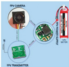
Fig. 8: FPV camera and transmitter setup (airborne)
