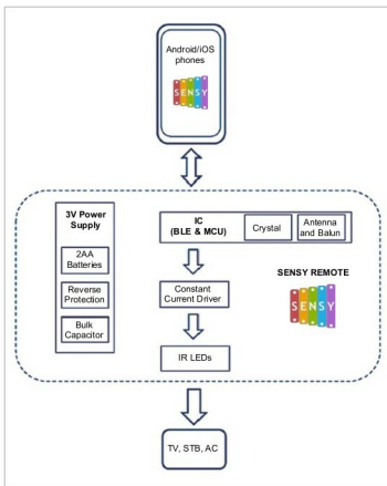
Block diagram for TV/STB/AC control from the smartphone using Sensy Remote
