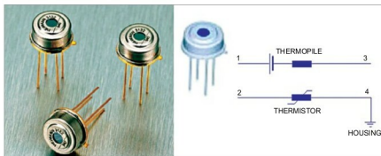
Fig. 4: (L) TPS334 package and (R) its pin drawing
