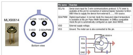
Fig. 6: Pin configuration of MLX90614
