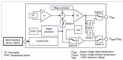
Fig. 5: Functional diagram of A2TPMI
