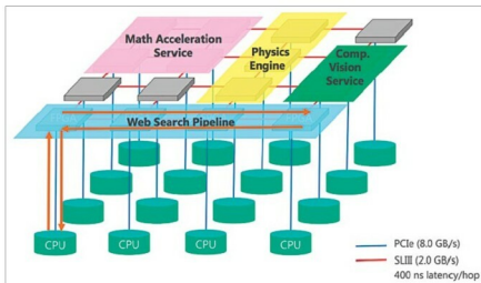
Fig. 19: Catapult uses a network of directly linked FPGAs
