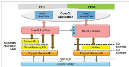
Fig. 24: OpenCL flow
