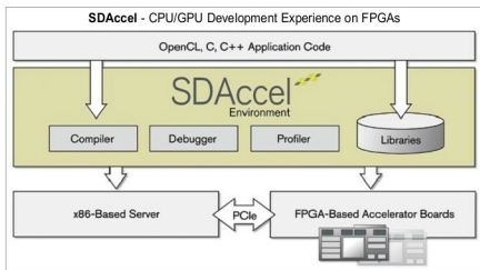
Fig. 25: SDAccel environment
