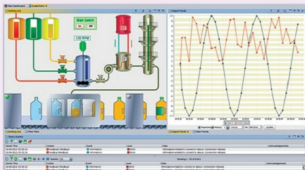
Fig. 5: HMI operator dashboard (Image courtesy: http://aggreagate.tibbo.com )
