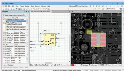
Fig. 4: Auto-cross probing (Image courtesy: www.altium.com )
