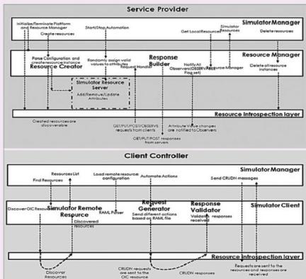
Fig. 3: Block diagram of service provider and client controller perspectives (Image courtesy: https://wiki.iotivity.org/iotivity_simulator )
