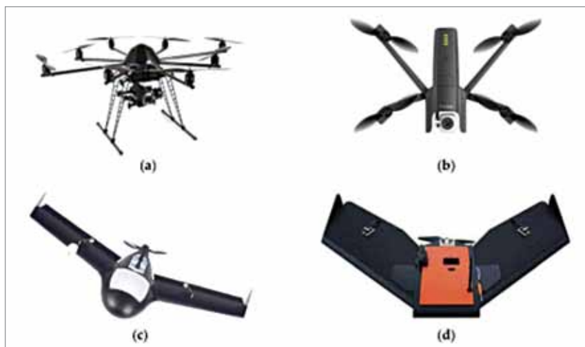
Fig. 3: Commercial drones used for precision agriculture purposes: (a) 8-rotor MK Okto XL 2 of HiSystems GmbH/Mikrokooper.de, (b) quad-rotor Parrot Anafi, (c) Gatewing X100, and (d) Tuffwing Mapper. P
