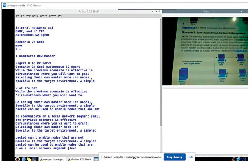
Fig. 3: Testing code
