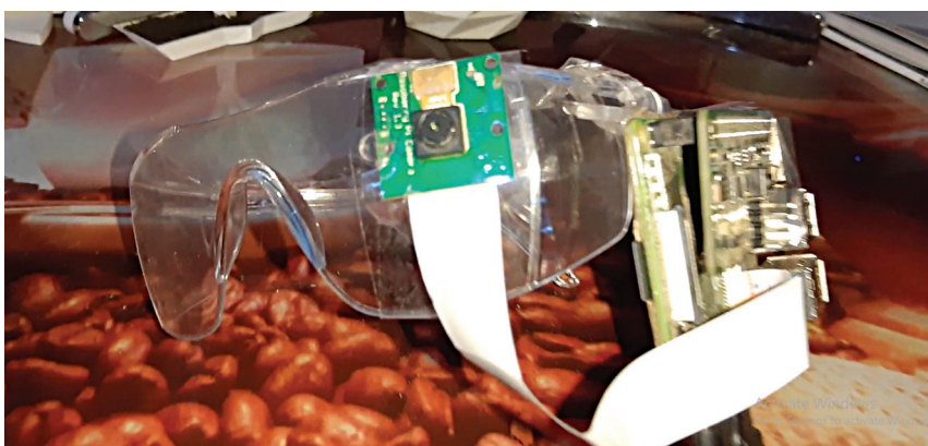
Fig. 4: Author's device attached with the camera on eyeglass
