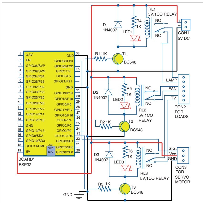
Fig. 4: Circuit diagram
