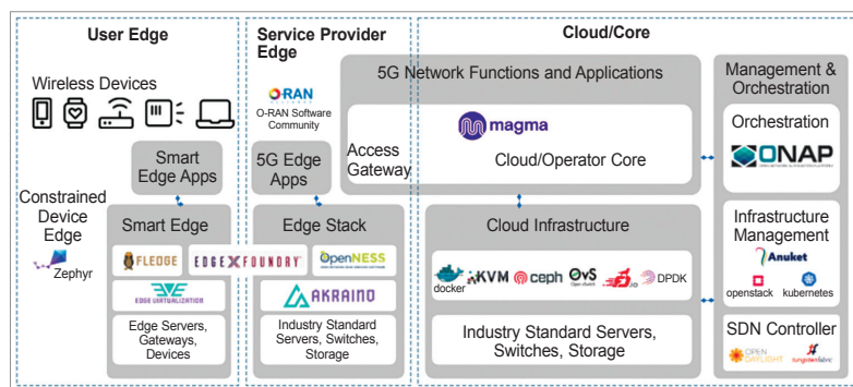
Fig. 1: LF open source component projects for 5G
