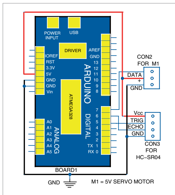
Fig. 2: Circuit diagram
