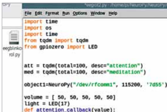
Fig. 4: Setting pin numbers for controlling lights, fans, etc
