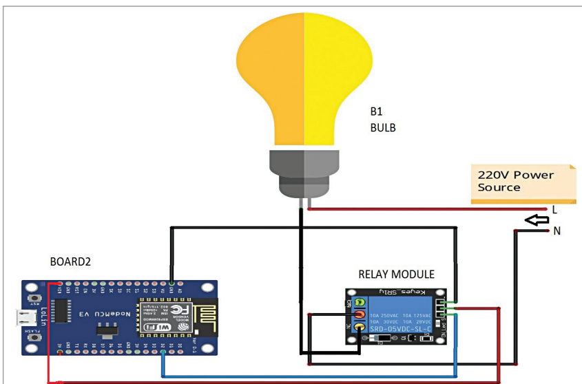
Fig. 2: Connection diagram of receiver
