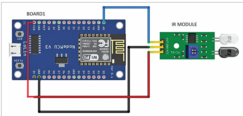
Fig. 1: Connection diagram of IR transmitter
