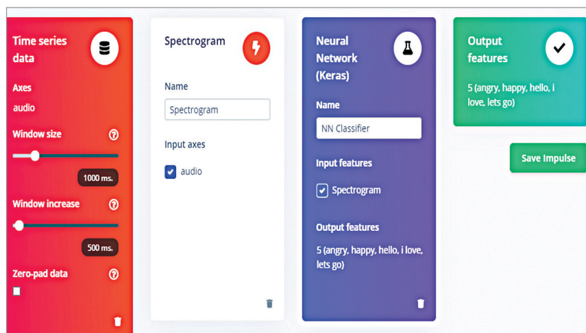
Fig. 3: Setting processing blocks
