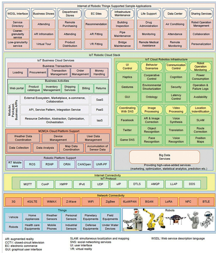
Conceptual diagram of IoRT (Source: Ray, Partha Pratim – Internet of Robotic Things: Concept, Technologies, and Challenges DOI 10.1109/ACCESS.2017.2647747)
