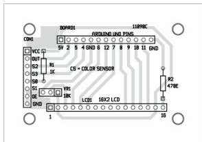
Fig. 7: Components layout of the PCB
