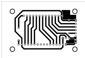
Fig. 6: Actual-size PCB layout of colour identification
