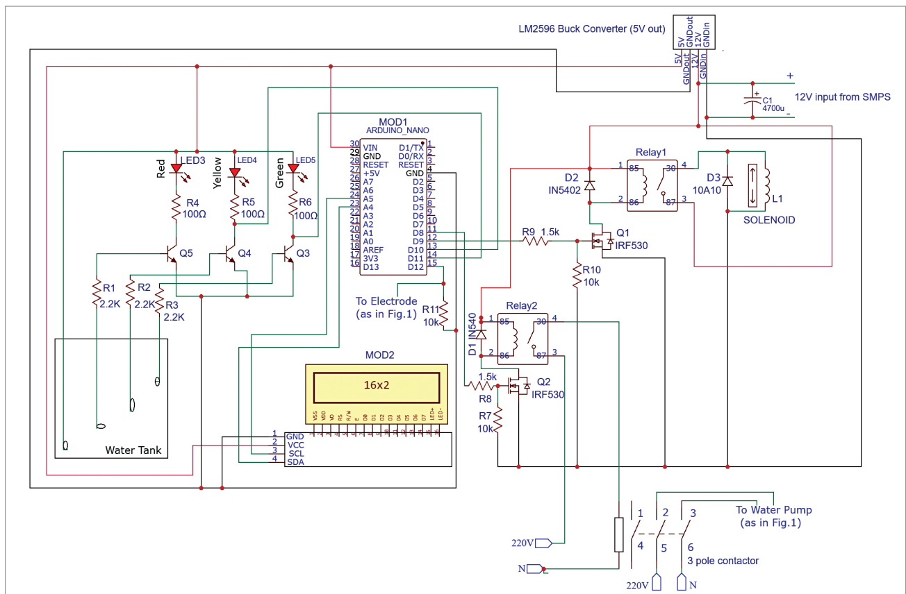
Fig. 2: Circuit diagram
