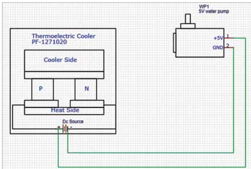
Fig. 13: Connection diagram of the project
