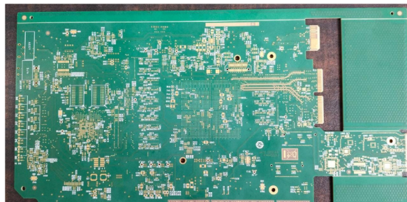
PCB 12 Layer, HDI, BGA, ENIG
