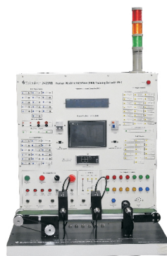
Human Machine Interface (HMI) with PLC
